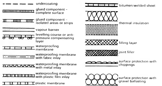
12 Key to representation of roof covering components
